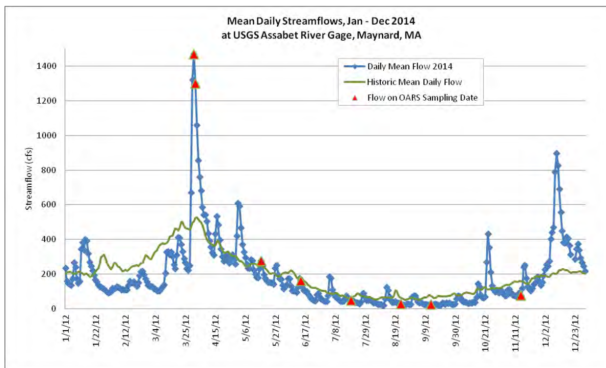
Figure 4: Mean Daily Streamflows Assabet River: 2014
