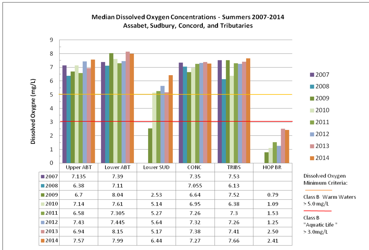
Figure 5: Median Dissolved Oxygen Measurements (Summers 2009 – 2014)
